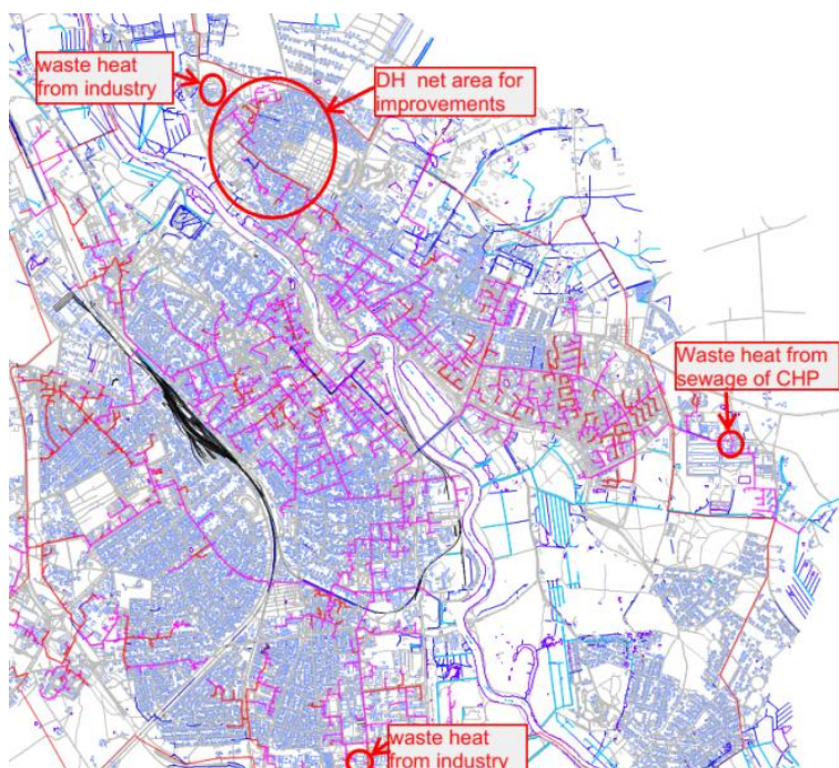
Figure 14. Overview Fortum DH network Tartu and potential distributed heat sources
